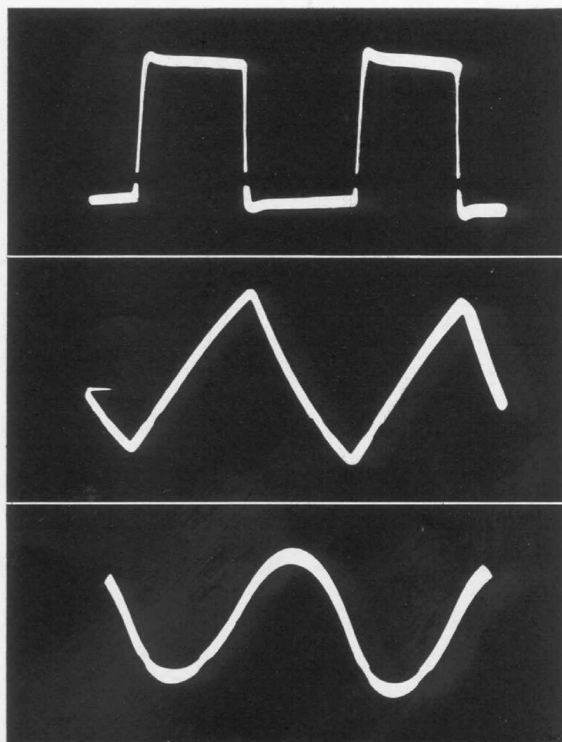
FIGURE 3. The action of the integrating circuits is shown by these oscillograms of the output voltage of the vibration meter for the three types of response when a square wave is applied to the input. At the top is shown the displacement response with wave shape unaltered; the velocity is shown at the center; and the lower oscillogram shows the acceleration.
